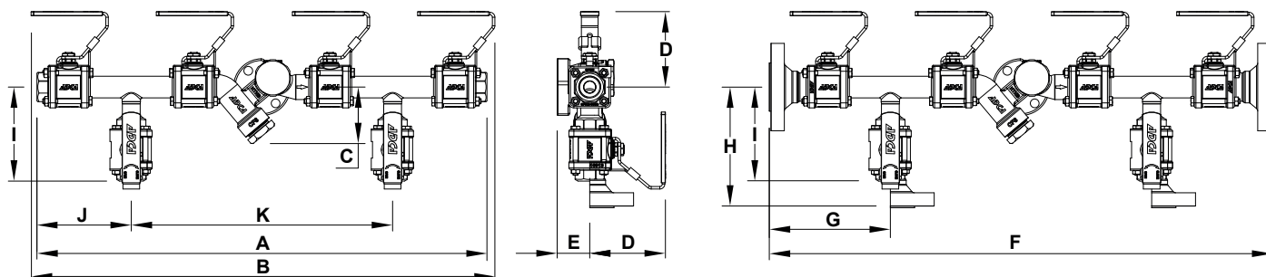
DIMENSIONS – CTS4UDB2 (mm)
