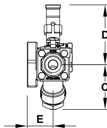
DIMENSIONS – CTS4U (mm)
