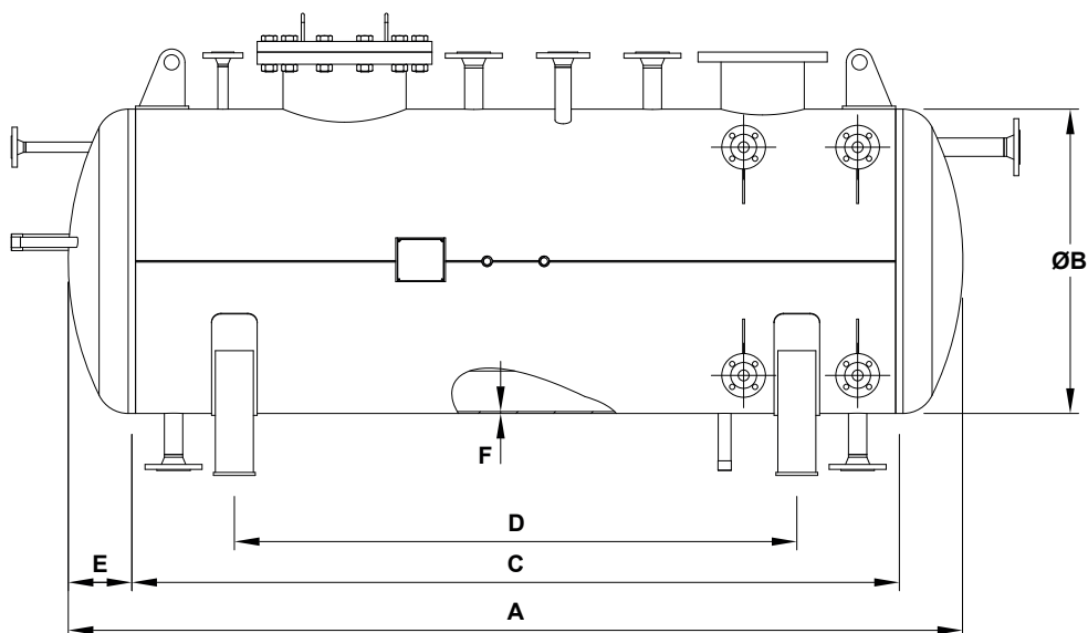
DIMENSIONS (mm)
