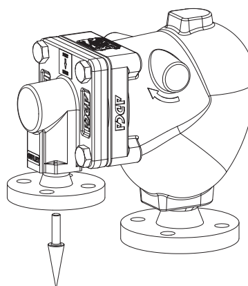
VB - Vertical inlet / top to bottom outlet
