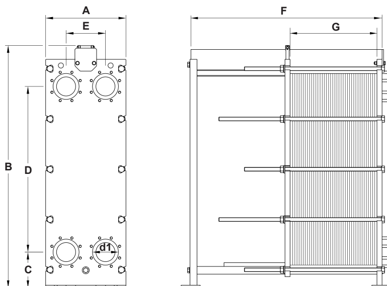
DIMENSIONS (mm)
