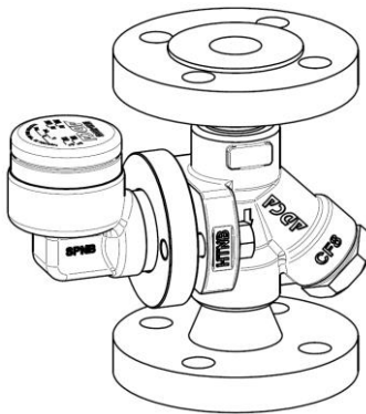
UDT steam trap connected to a UCX universal pipeline connector
