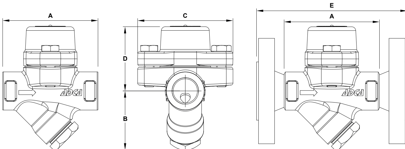
DIMENSIONS (mm)
