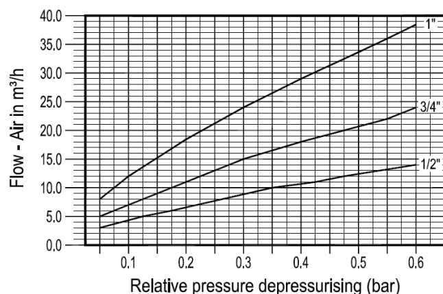
CAPACITY CHART
