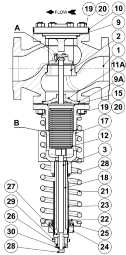
DN 65 – DN 100
