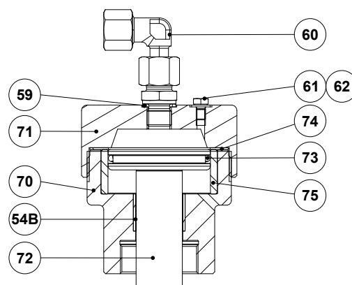
P series actuators
