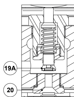
Detail A Pilot valve (soft)
