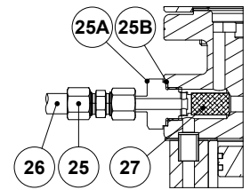
Optional external sensing line connection
