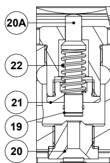
Detail A Pilot valve
