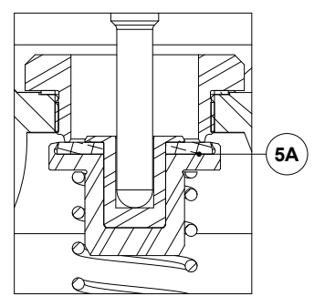
Detail B Main valve (soft)
