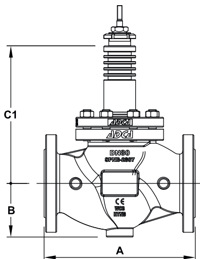
Valve with extended bonnet
