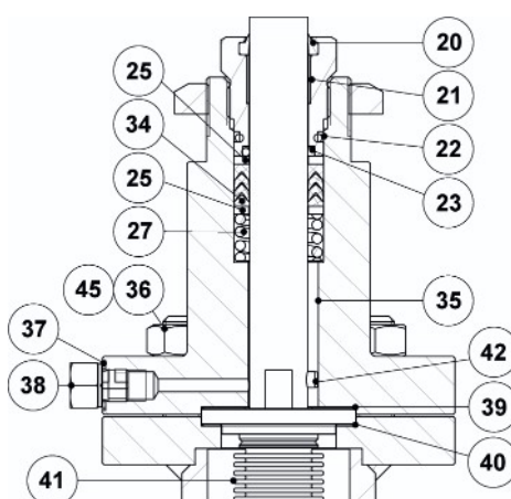
Bellows sealing (BV1)
