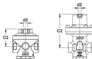
Optional dome-loaded version
