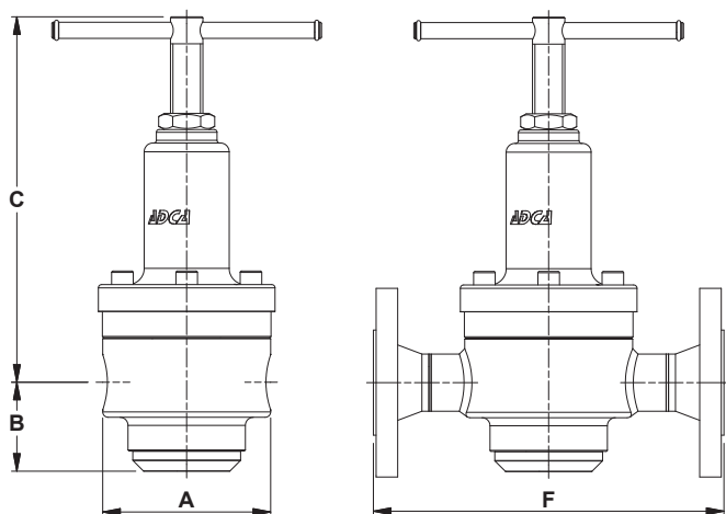
1" and 1 1/4" – DN 25 and DN 32
