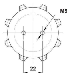
Optional bottom mounting connection
