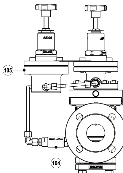
Fig. 8 - Pressure reducing and sustaining valve
