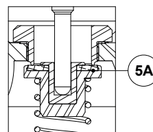
Detail B Main valve (soft)
