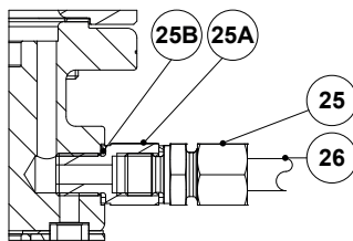
External sensing line connection
