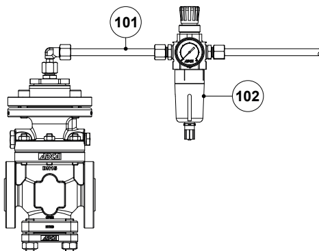
Dome-loading valve
