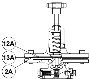
Optional low pressure diaphragm
