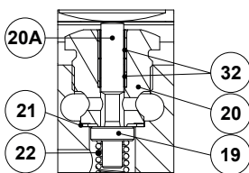
Detail A Pilot valve
