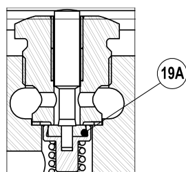
Detail A Pilot valve (soft)
