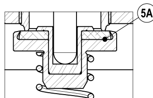
Detail B Main valve (soft)
